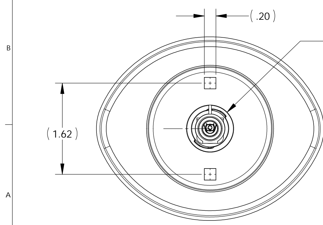
BACK VIEW
